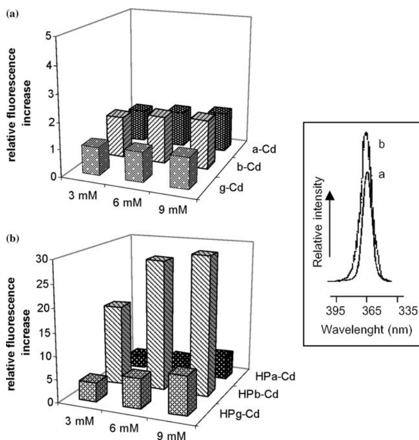
Figure 2. Relative fluorescence increase of 0.4 mM triclosan (TRI) aqueous solution in the presence of increasing concentrations of natural (a) or hydroxypropyl derivative (b) cyclodextrins. The fluorescence spectra of TRI alone (a) and in the presence of 6mM \alpha Cd (b) are shown in the window as an example.
