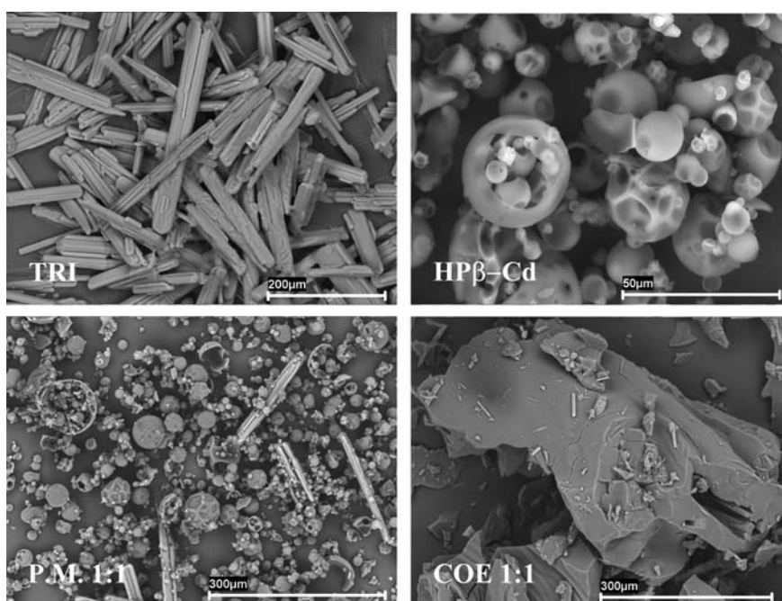
Figure 6. SEM micrographs of pure TRI, HP\beta -Cd and their PM, KN and coevaporated (COE) products.
