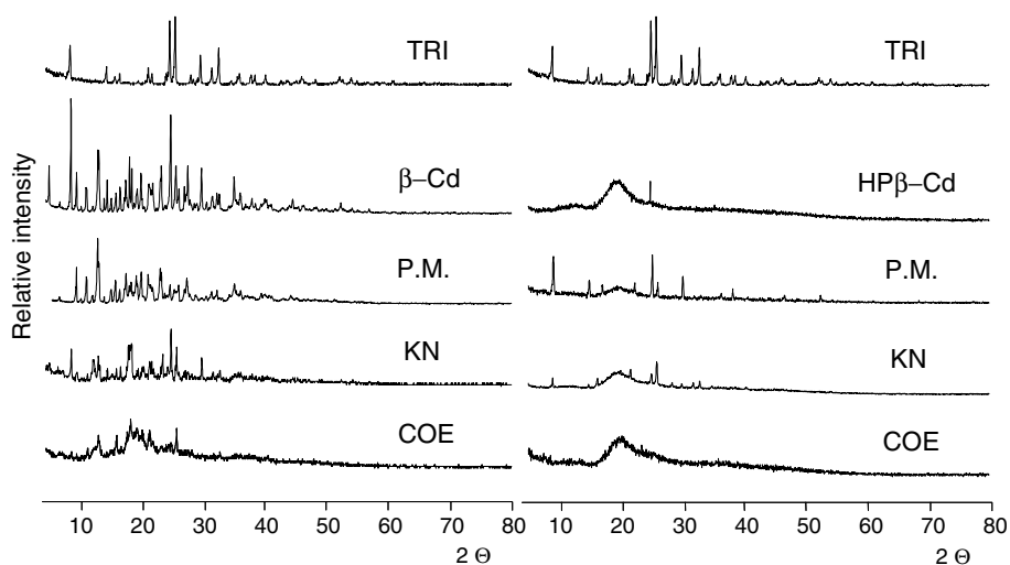
Figure 5. X-ray powder diffraction patterns of pure TRI, \beta -Cd, and HP\beta -Cd, and their equimolar PM, KN and COE products.
