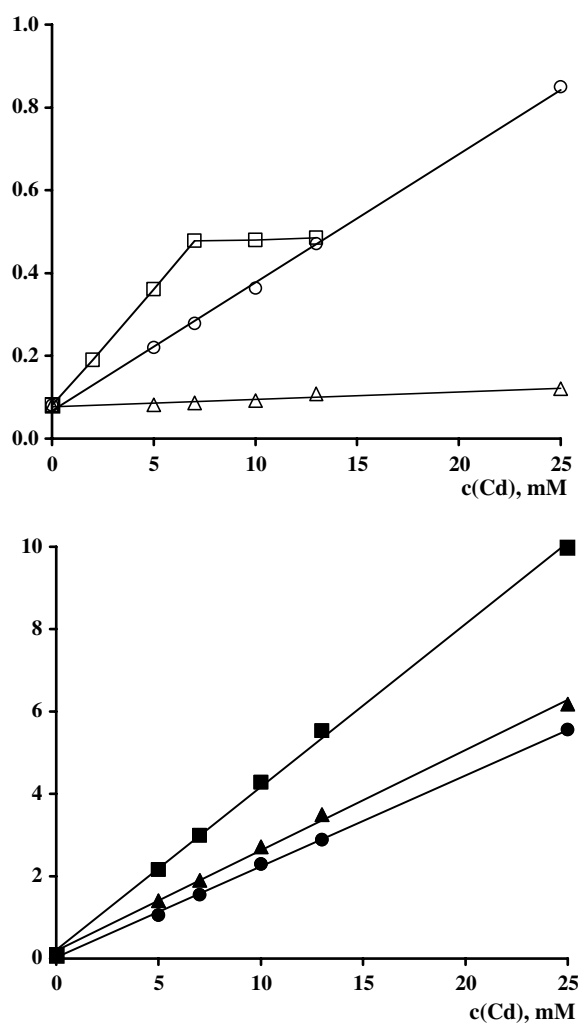
Figure 1. Phase-solubility diagrams in aqueous solutions at 25 \pm 0.5 °C of TRI in the presence of natural (a) or hydroxypropyl derivative ( \beta ) cyclodextrins. Key (a): \alpha -Cd ( \diamond ), \beta -Cd ( \square ), \gamma -Cd ( \triangle ); (b): HP \alpha -Cd ( \blacklozenge ), HP \beta -Cd ( \blacksquare ), HP \gamma -Cd ( \blacktriangle ).
