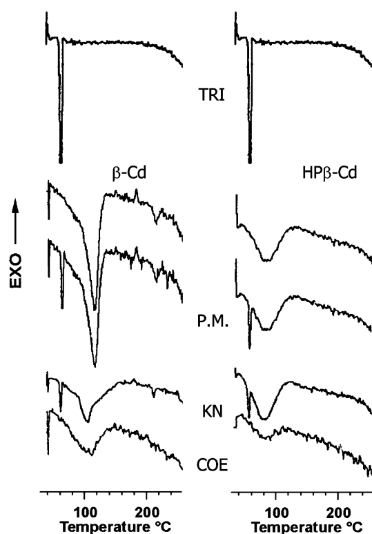
Figure 4. DSC curves of pure TRI, \beta -Cd, and \text{HP}\beta -Cd, and their equimolar physical mixtures PM, kneaded KN and coevaporated COE products.
