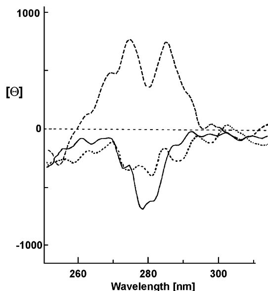
Figure 3. Circular dichroism absorption spectra of TRI alone (unbroken line) or in the presence of 6 mM \alpha -Cd (dotted line) and \beta -Cd (broken line).
